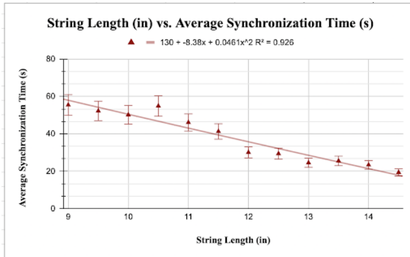
Figure 6: This is the string length (in) vs. average synchronization times (s) graph taken directly from the data table(s) shown above. The graph includes a polynomial approximation (appears linear) as demonstrated by the equation and line of best fit which has a R^2 value of 0.926 which indicates the correlation is very strong. The polynomial and linear approximations give the same R^2 value, but the polynomial representation is picked. The error bars present on the graph seem to get smaller as the string length increases in length. Overall, the graph represents an inverse polynomial decreasing relationship between the two variables.
