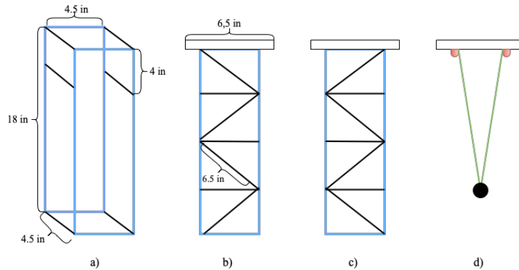
Figure 2: The blue lines designate the thick balsa wood sticks, black lines designate the thin balsa wood sticks, green lines designate string, red lines indicate staple hooks, and the thin rectangles are the small wooden planks a) A simplified (doesn't have cross supports) cartoon 3D depiction of the dimensions of the tower (with measurements), including what the sides look like b) The front side of the tower which contains the wooden bar c) The back frame of the tower, the diagonal supports are in the opposite direction of the front frame d) The depiction of how the pendulum bob hangs on the metal hooks (The bob is hooked onto the string).
